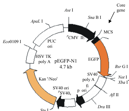
Fig.2 Schematic representation of different plasmid construction: Different truncated CORE were inserted into MCS: Nhe I and Eco I to yield CORE-GFP fusion protein expression plasmids
